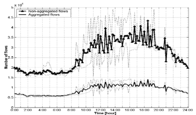
Fig. 2 Size of the original and the aggregated data sets over one day
